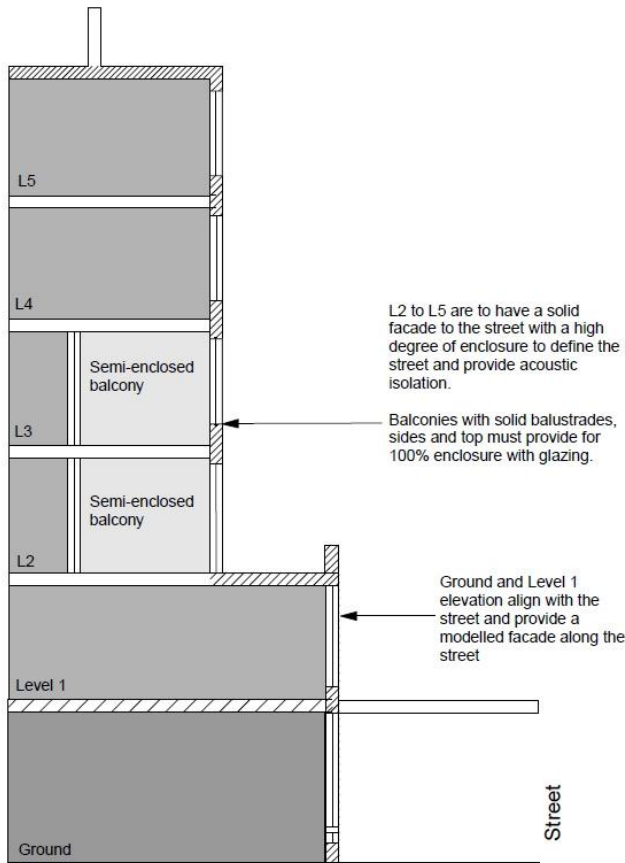
Figure 28 Façade section
