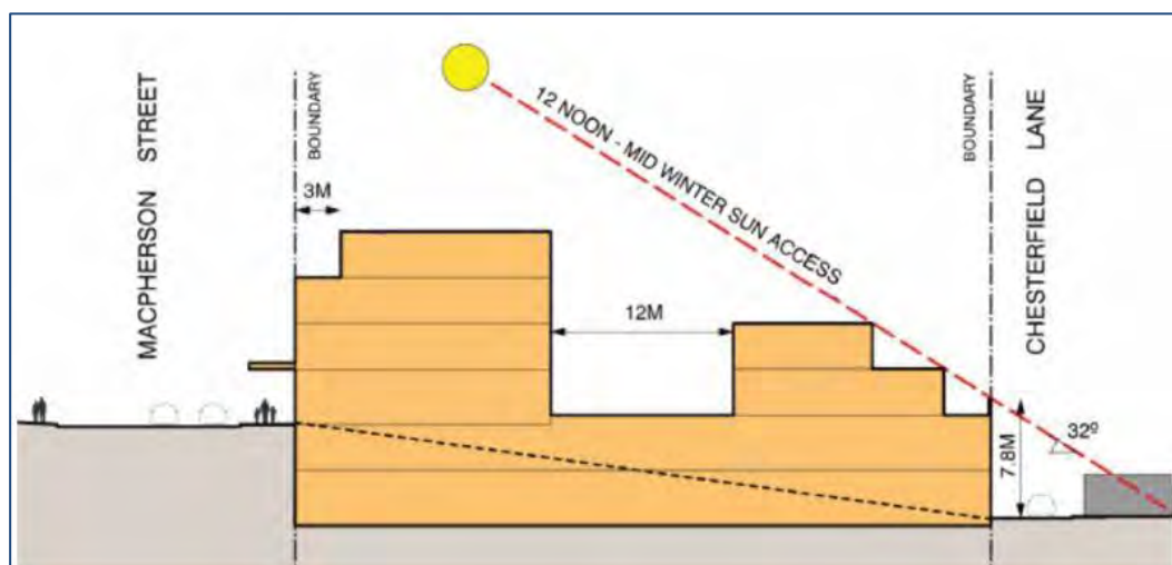
Figure 59 Development Control Envelope section
