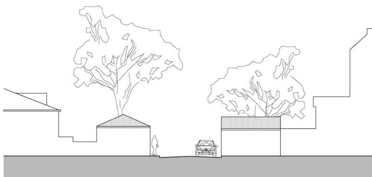
Figure 43 Typical section of a rear access lane.
