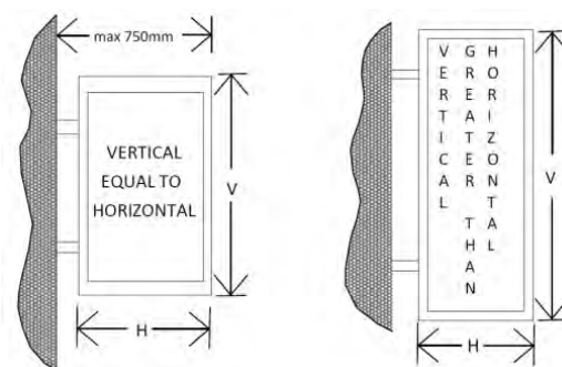
Figure 29 Dimensions for vertical projecting wall signs
