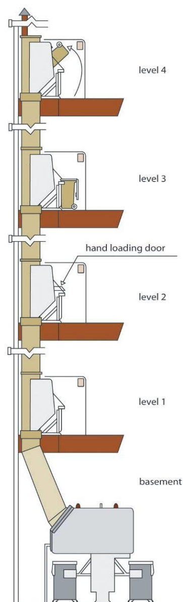
Example of a garbage chute system
