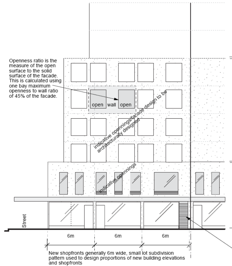
Figure 27 Elevations
