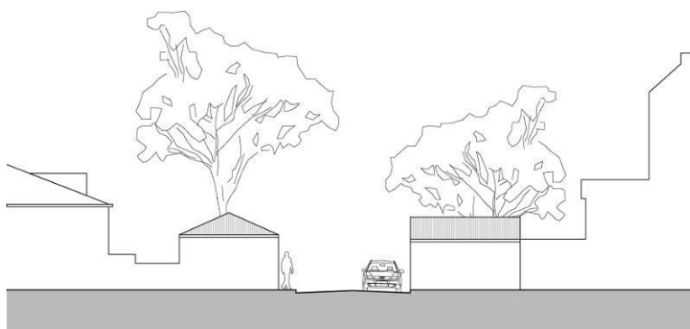
Figure 28 Typical section of a rear access lane.
