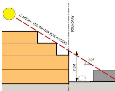
Figure 56 Setbacks at rear lanes to ensure solar access to neighbours
