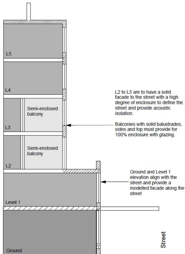
Figure 28 Façade section
